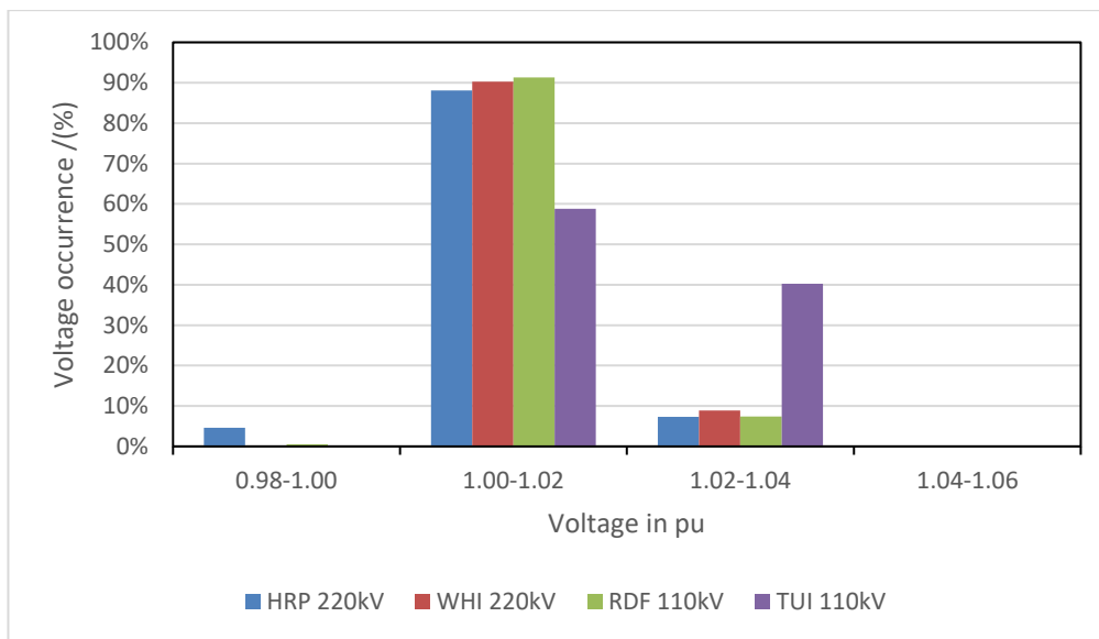
Figure 3-1: Voltage profile of HRP220kV, WHI20kV, RDF110kV, and TUI 110kV from Jan to Dec 2024
