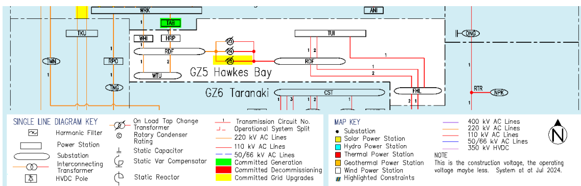
Figure 1-2: Single line diagram of Hawkes Bay Region (Grid Zone 5)
