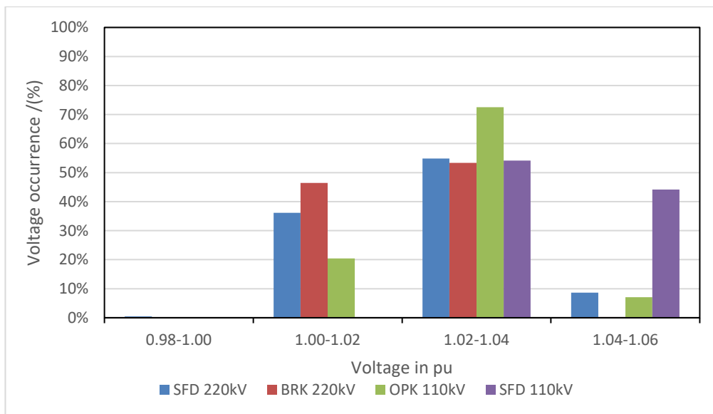
Figure 3-1: Voltage profile of SFD 220kV, BRK220kV, OPK110kV, and SFD110kV from Jan to Dec 2024
