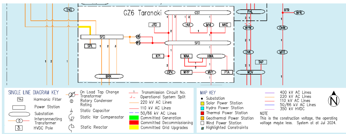
Figure 1-2: Single line diagram of Taranaki Region (Grid Zone 6)
