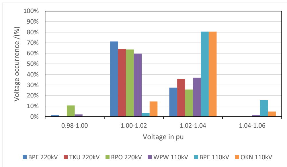
Figure 3-1: Voltage profile of BPE220kV, TKU220kV, RPO220kV, WPW110kV, BPE110kV and OKN110kV from Jan to Dec 2024
