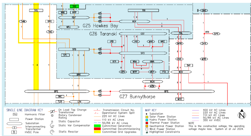
Figure 1-2: Single line diagram of Bunnythorpe Region (Grid Zone 7)
