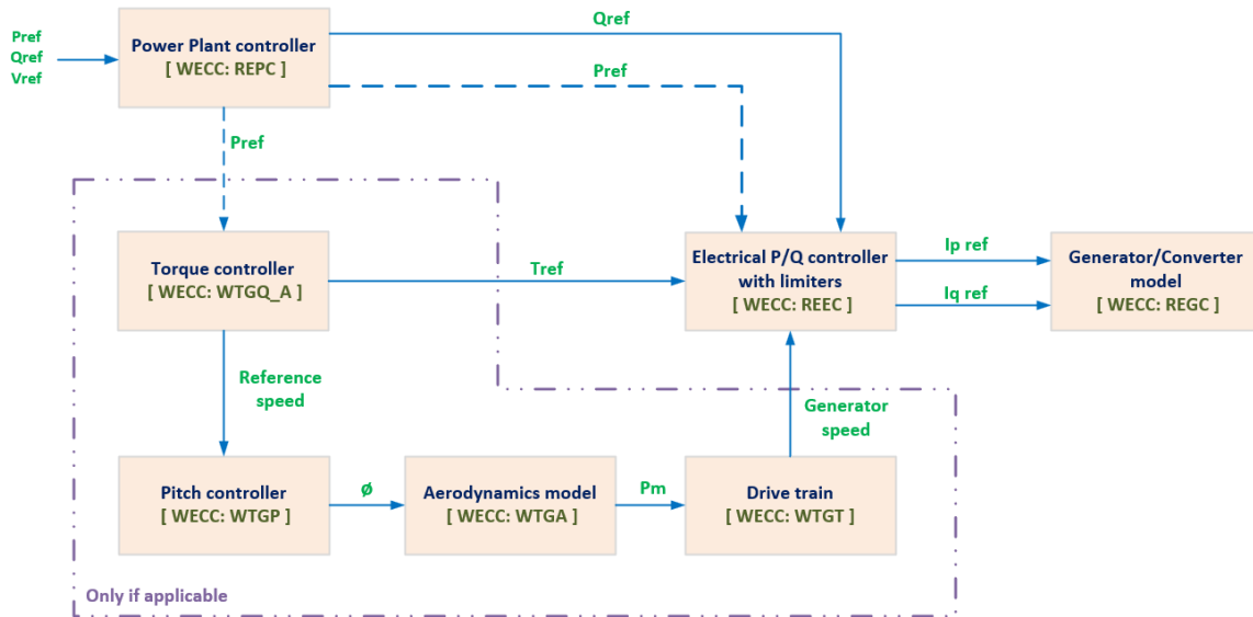
Figure 5 : Typical Components of an IBR Control System &amp; their Equivalent WECC Model
