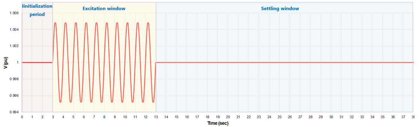
Figure 9: Typical Simulation Window for 1 Hz Voltage Oscillation
