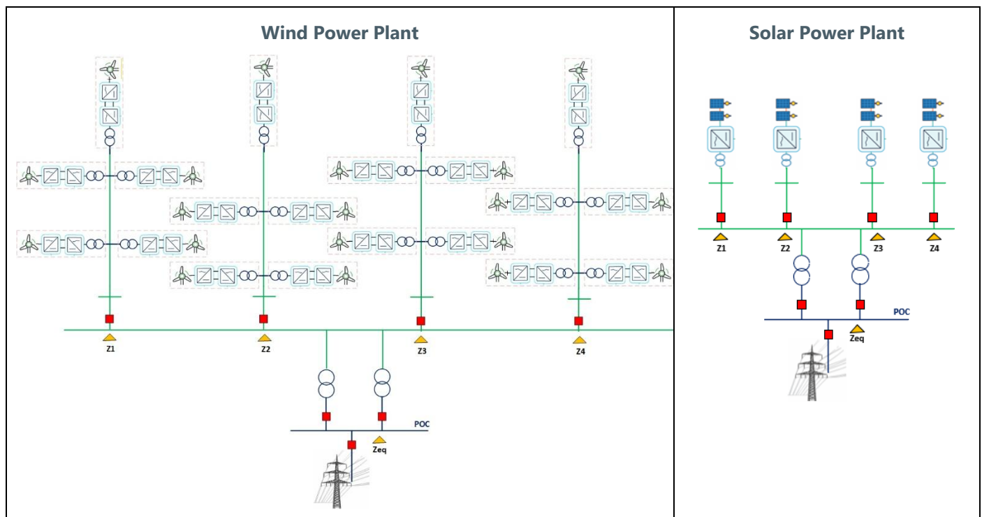
Figure 11: Typical Grid-connected IBR Arrangements
