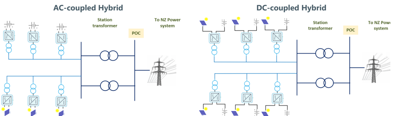
Figure 3: Typical Hybrid IBR Stations
