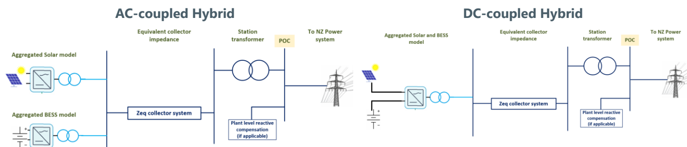
Figure 4: Typical Aggregation of Hybrid Stations
