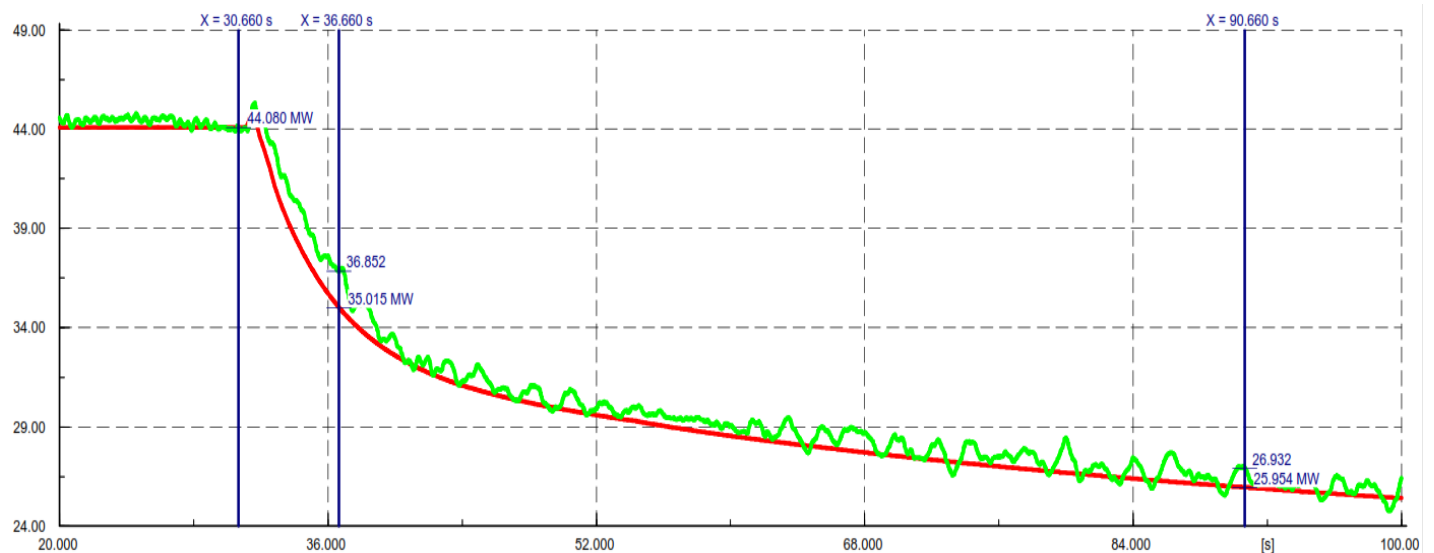
Figure 10: Example Plot showing 'Good Fit' between Model Performance and Test Results
