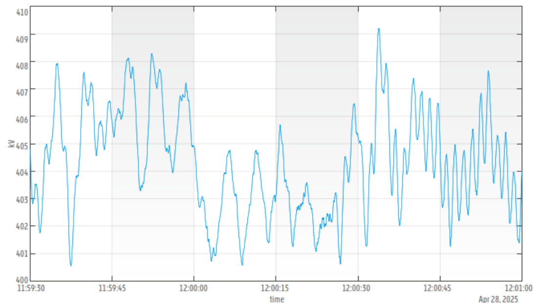
0.63 Hz voltage oscillations prior to the event. Source: ENTSO-E final report
