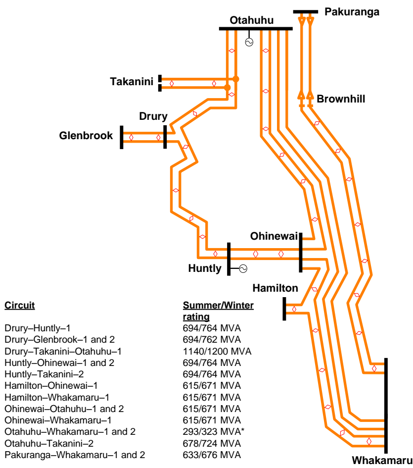
Figure 6-5: 220 kV Upper North Island grid backbone circuits
