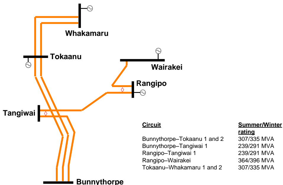
Figure 6-8: 220 kV Central North Island circuits
