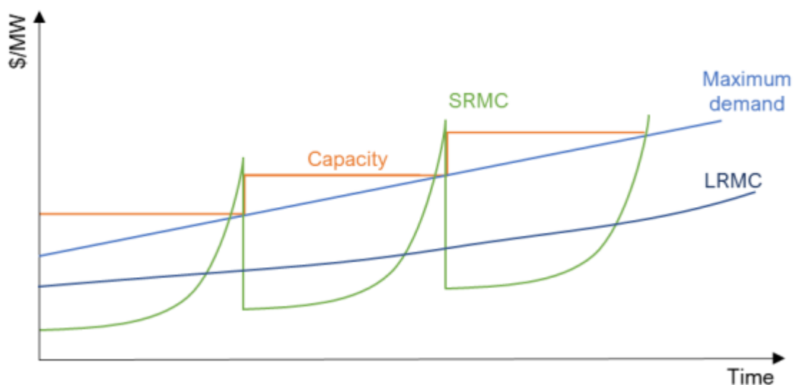
Figure 1: Simple illustration of how SRMC and LRMC develop as maximum demand increases
